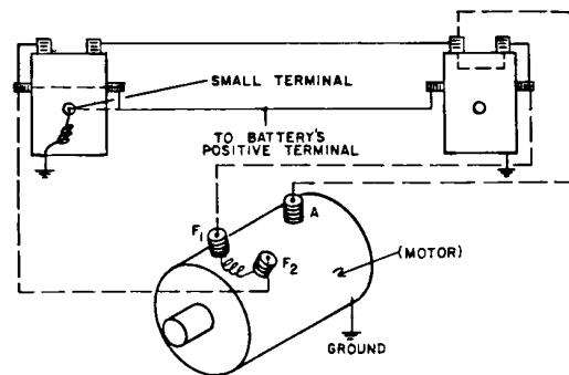
FIGURE -2 MOTOR - COUNTER CLOCKWISE ROTATION
